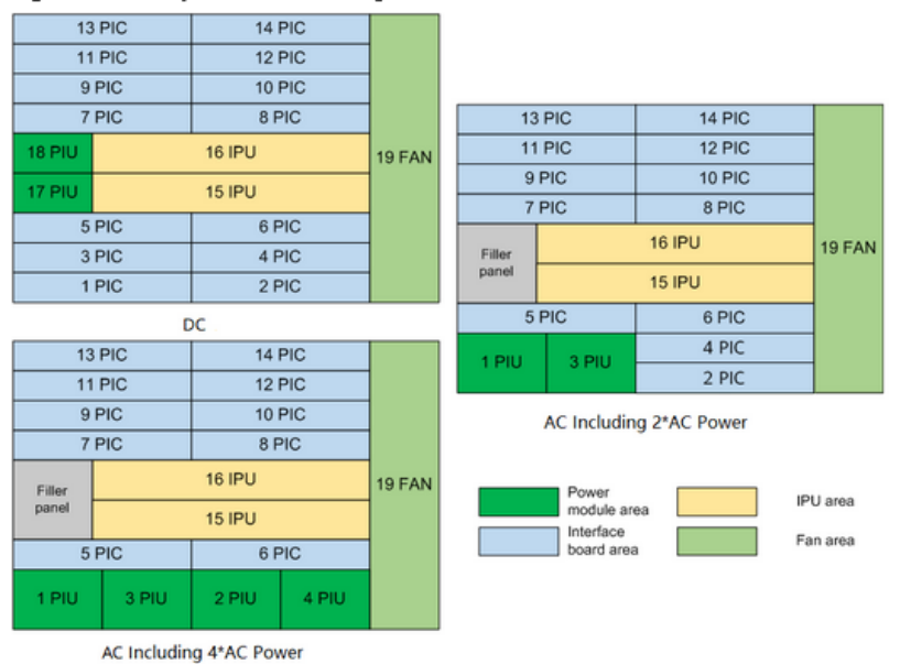
Figure 7 Slot Layout of the NetEngine 8000 M14
